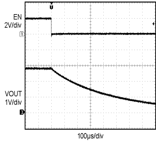
Figure 15. Enable Turn-off (100 \mu\text{A} Load)
