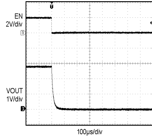
Figure 17. Enable Turn-off (500 mA Load)
