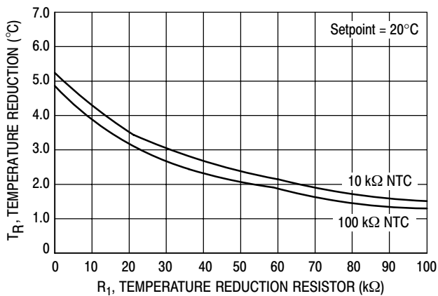
Figure 14. Temperature Reduction versus R_1
