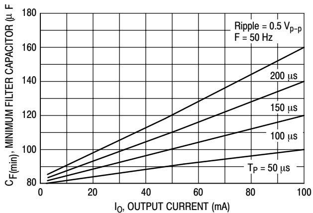
Figure 13. Minimum Filter Capacitor versus Output Current
