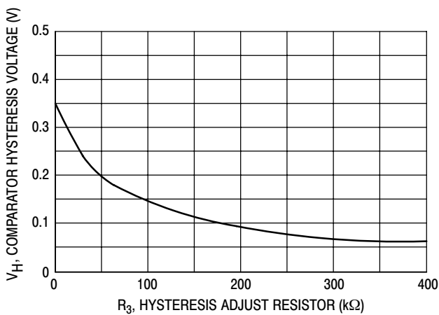
Figure 18. Comparator Hysteresis versus R_3
