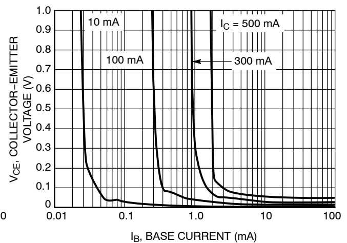
Figure 20. Saturation Region
