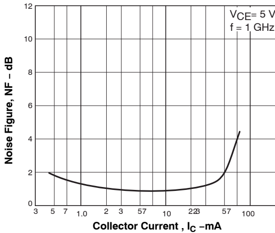
Figure 5. NF - I_C
