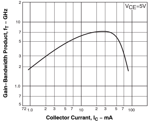
Figure 2. f_T - I_C
