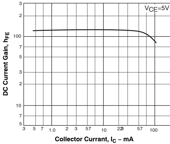
Figure 1. h_{FE} - I_C
