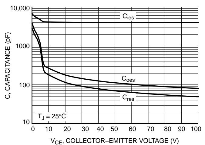
Figure 6. Typical Capacitance
