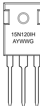
TO-247 CASE 340AL
