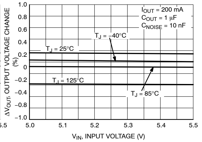
Figure 6. Line Regulation
