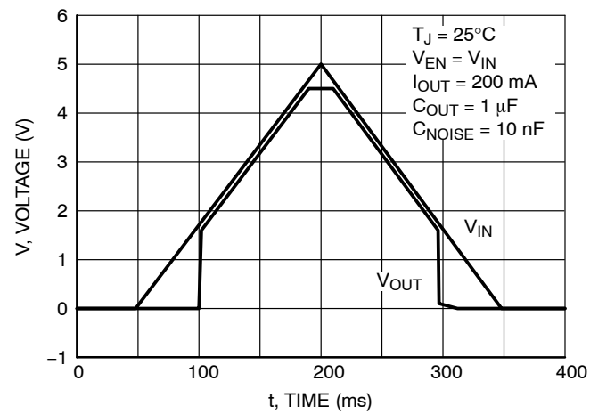
Figure 32. Power-Up / Down
