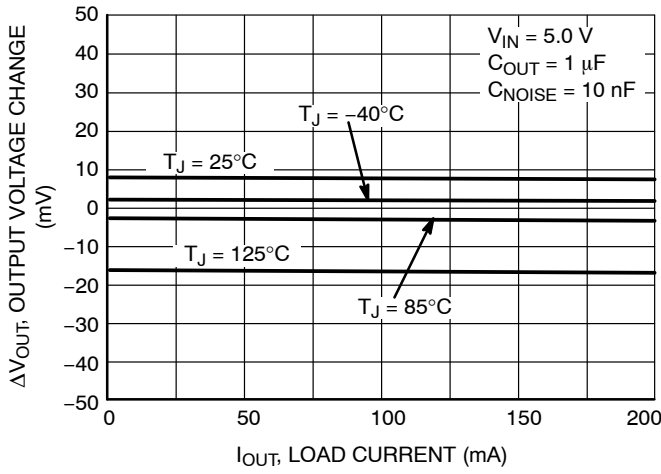
Figure 3. Load Regulation
