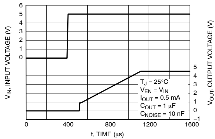
Figure 31. Power-Up
