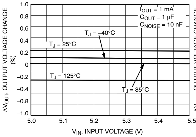
Figure 5. Line Regulation
