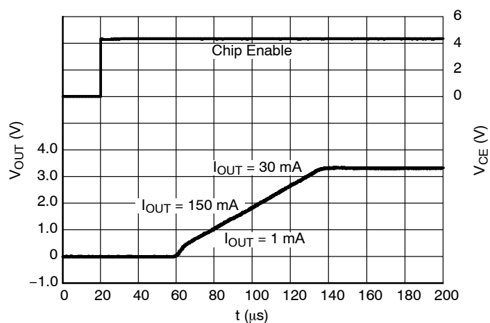
Figure 35. Start-up, 3.3 V Version, V_{\text{IN}} = 4.3 \text{ V}
