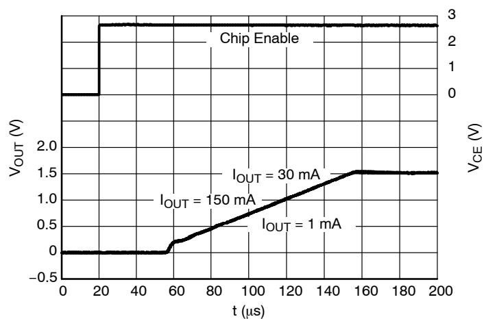
Figure 34. Start-up, 1.5 V Version, V_{\text{IN}} = 2.6 \text{ V}
