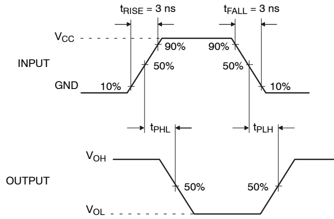
Figure 7. AC Waveforms
