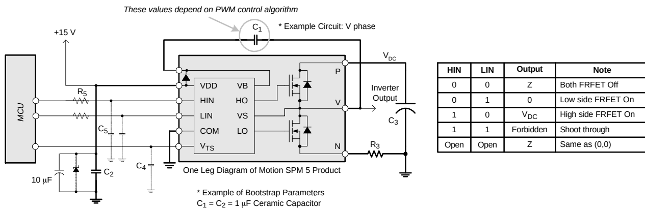
Figure 4. Recommended MCU Interface and Bootstrap Circuit with Parameters
