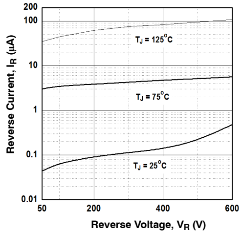
Figure 20. Reverse Current
