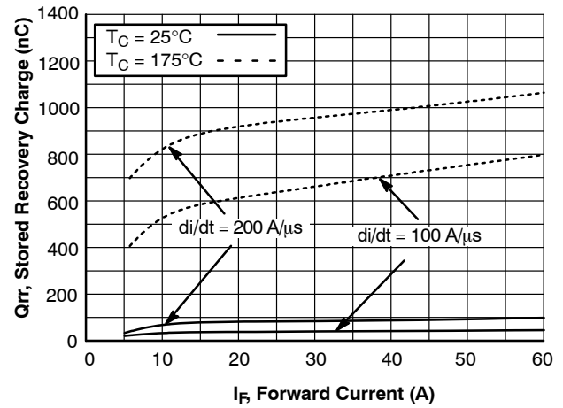
Figure 20. Stored Charge
