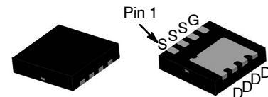
WDFN8 3.3 x 3.3, 0.65P CASE 511DH
