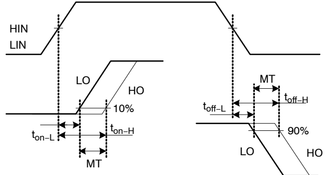
Figure 35. Delay Matching Waveform Definition
