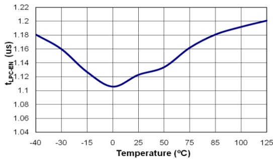
Figure 15. Minimum LPC Enable Time
