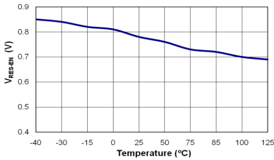
Figure 13. Threshold Voltage of V_{RES}
