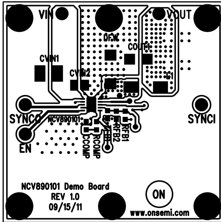
Figure 16. Top View
