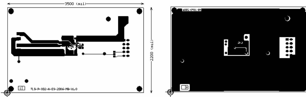
Figure 4. NCP5612GEVB Evaluation Board: TOP & BOTTOM Views
