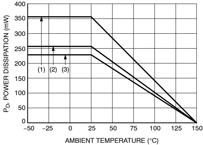
Figure 130. Derating Curve
