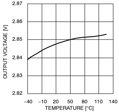
Figure 6. Output Voltage vs. Temperature
