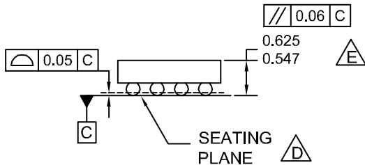
SIDE VIEWS
