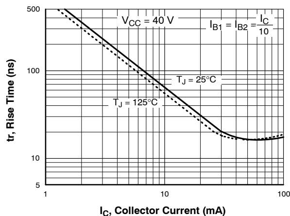
Figure 12. Rise Time vs. Collector Current
