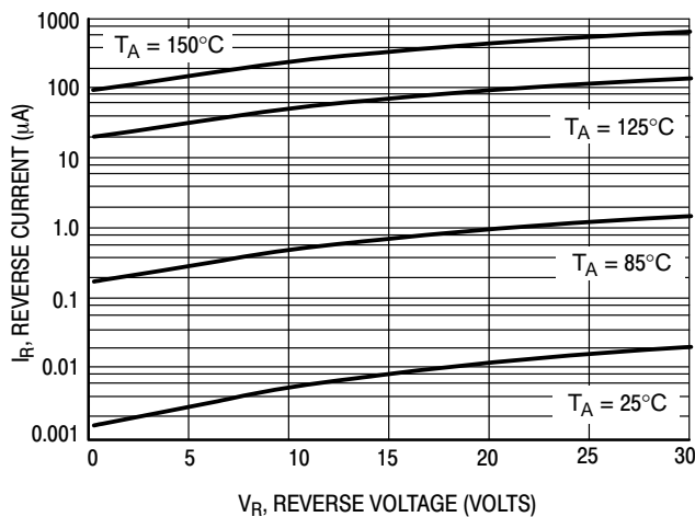
Figure 3. Leakage Current
