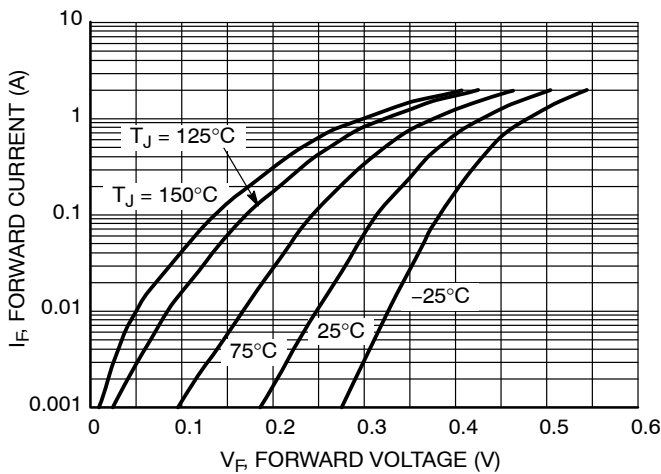
Figure 1. Forward Voltage
