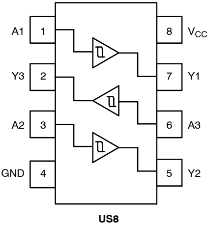
Figure 2. Pinout
