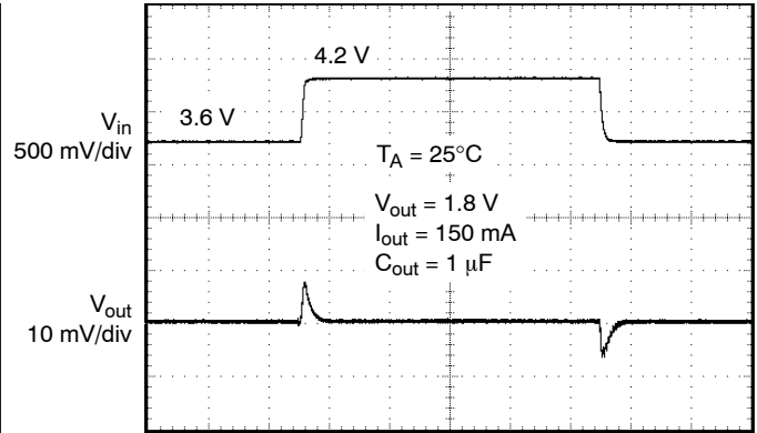
Figure 21. Line Transient
