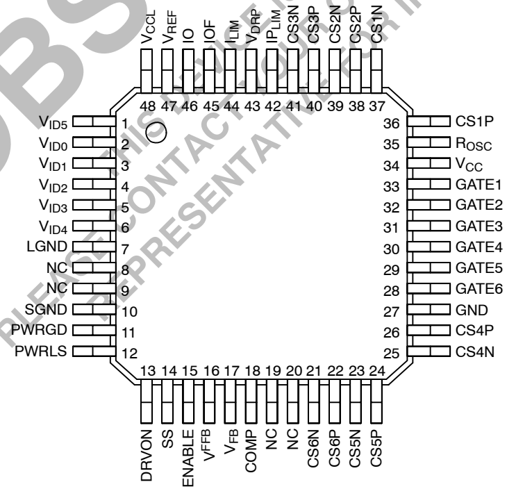
LQFP-48
