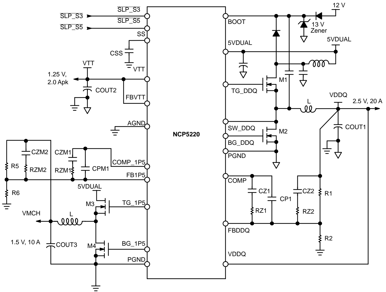
Figure 1. Application Diagram
