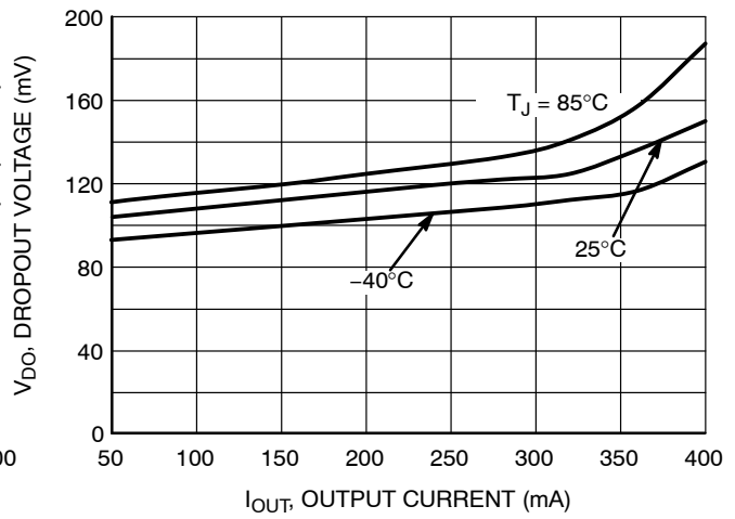
Figure 34. Dropout Voltage vs. Output Current 1.0 V Version
