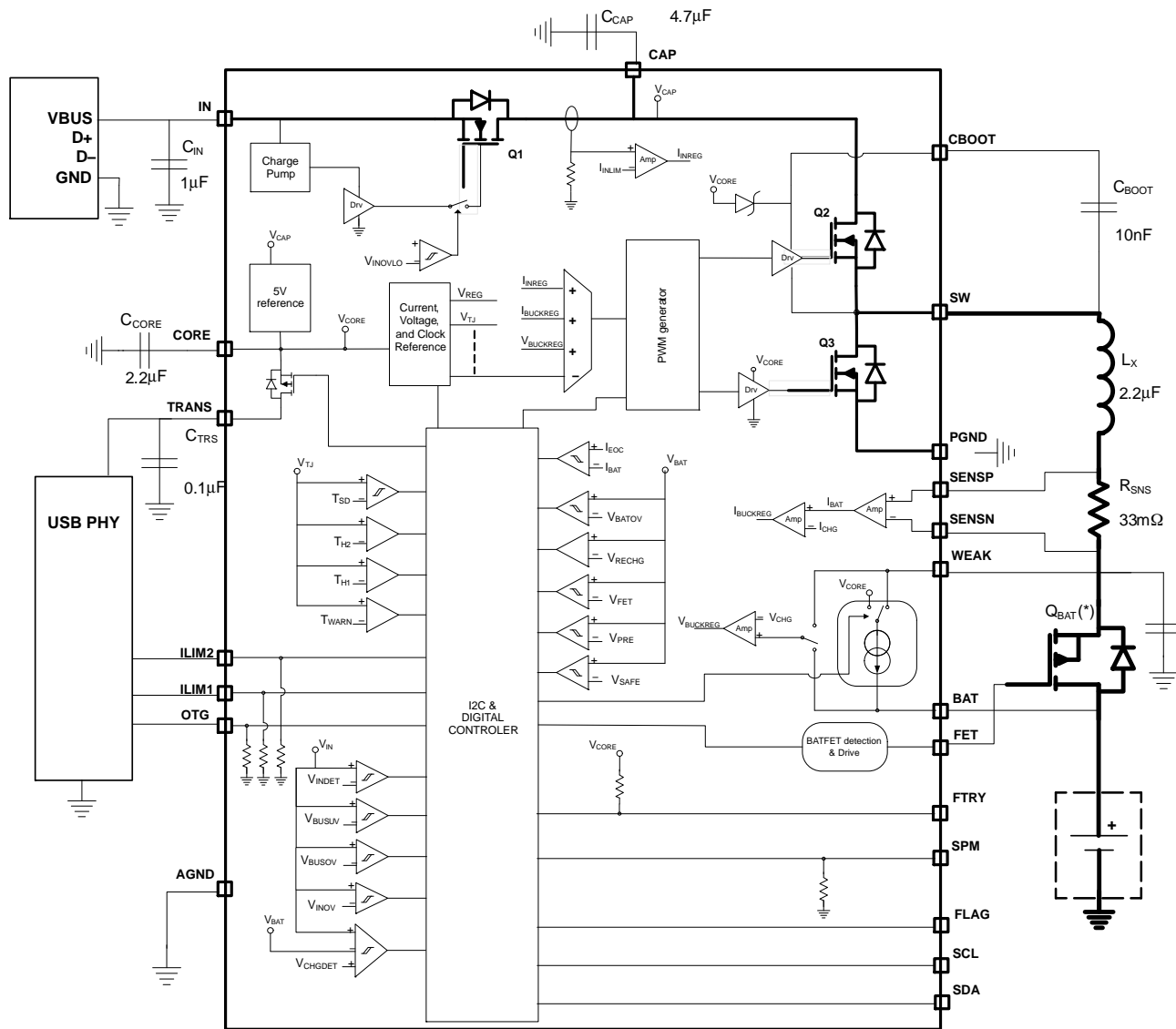
Figure 4. Block Diagram
