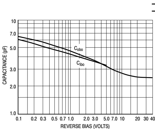
Figure 1. Capacitance
