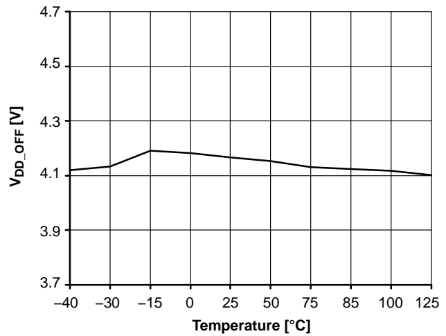
Figure 4. V DD_OFF
