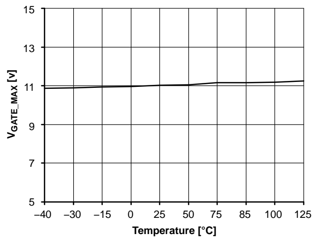
Figure 18. V_{GATE\_MAX}
