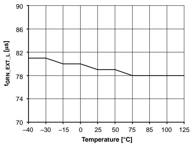
Figure 16. t_{GRN\_EXT\_L}
