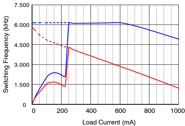
Figure 34. Frequency vs. Load Current to Demonstrate t_{OFF(MIN)} Effect, V_{IN} = 2.3 \text{ V} and 2.7 \text{ V} , V_{OUT} = 1.82 \text{ V} , Auto Mode, FPWM Dotted
