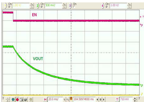
Figure 26. Shutdown, 10 \text{k}\Omega Load, No Output Discharge
