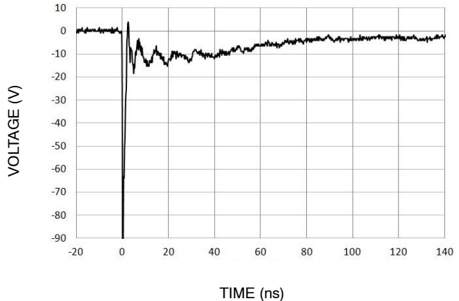
Figure 3. IEC61000-4-2 -8 kV Contact ESD Clamping Voltage
