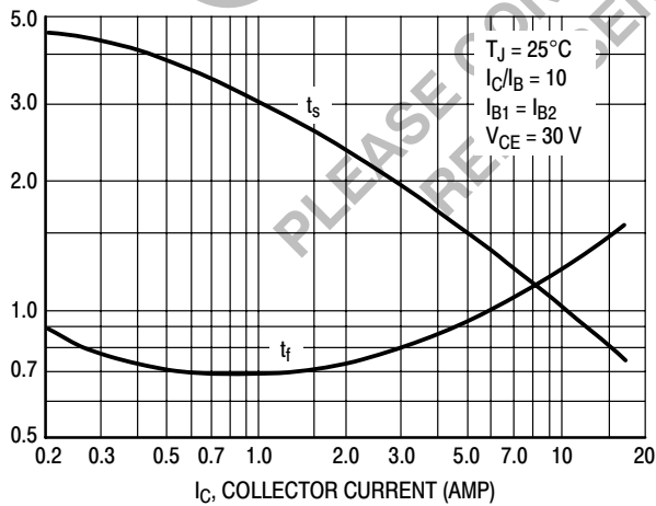
Figure 6. Turn-Off Time
