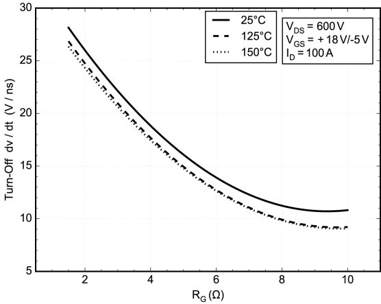
Figure 28. dv/dt OFF vs. R G
