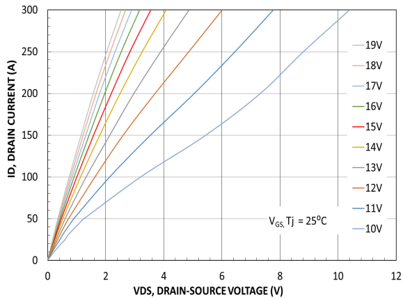
Figure 2. MOSFET Typical Output Characteristics
