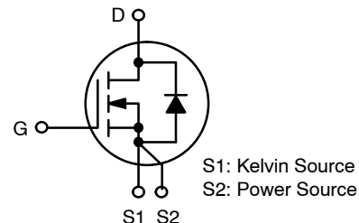
N-CHANNEL MOSFET
