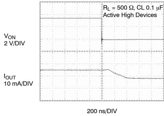
Figure 19. T OFF Response
