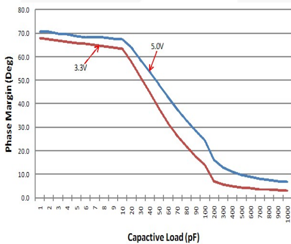
Figure 15. Phase Margin vs. Capacitive Load
