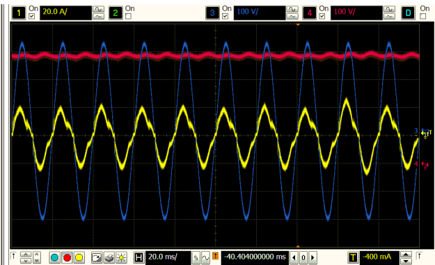
Figure 23. Vin 220 V, Pin = 3.3 kW
