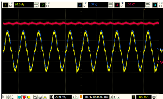
Figure 22. Vin 120 V, Pin = 3.3 kW
