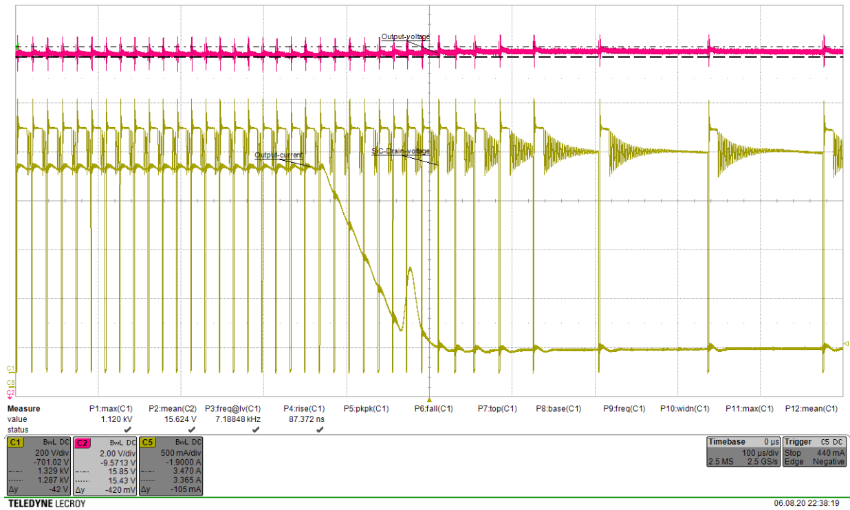
Figure 17. 900 V – 85% to 15%
