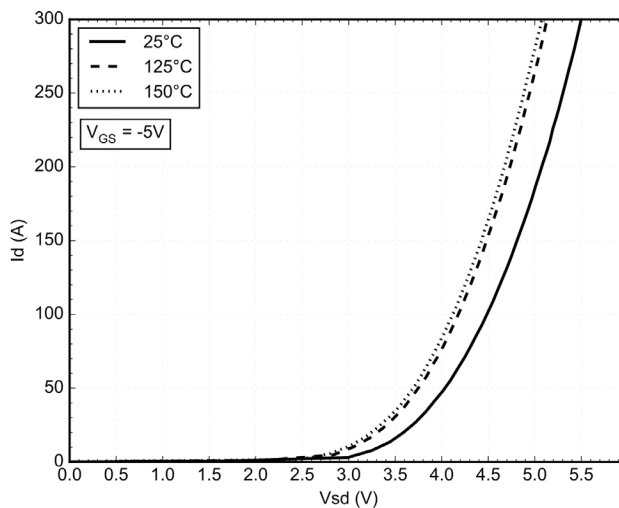
Figure 5. Body Diode Forward Characteristic
