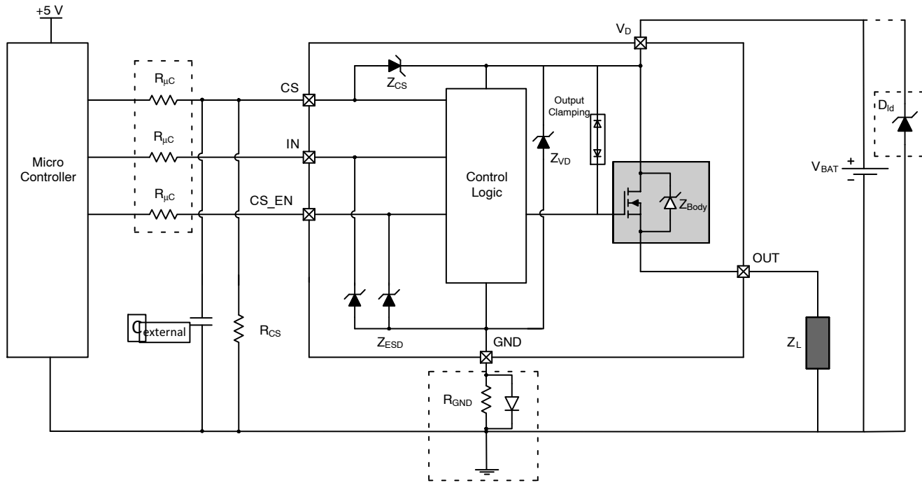
Figure 33. Application Schematic
