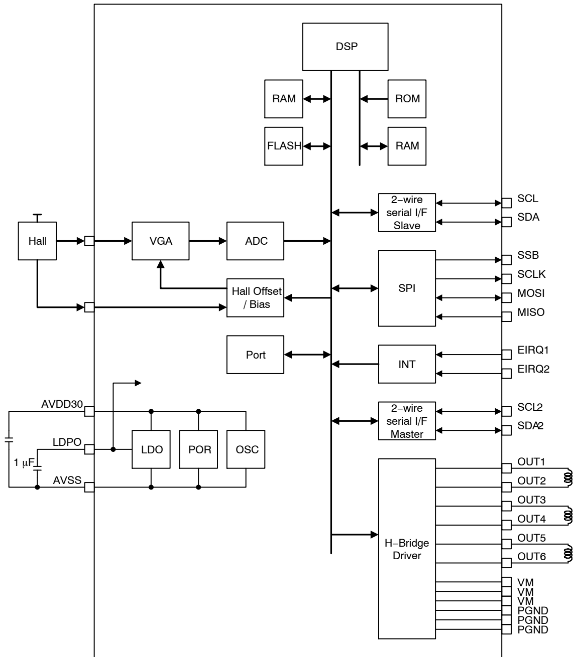
Figure 1. Block Diagram
