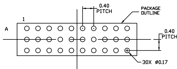
RECOMMENDED MOUNTING FOOTPRINT
