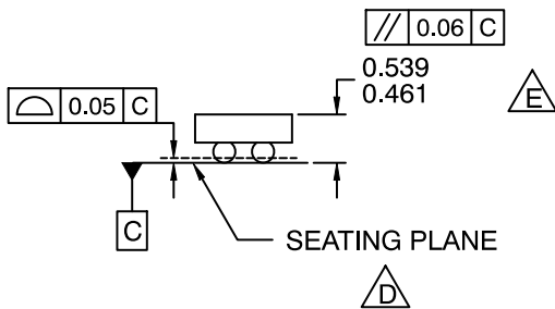
SIDE VIEWS
