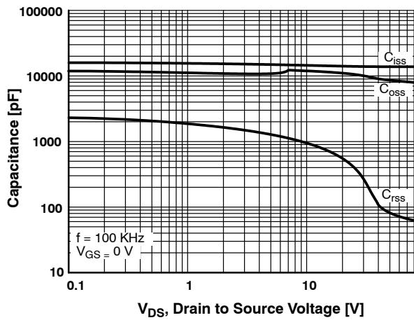
Figure 13. Capacitance Variation
