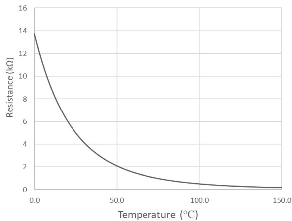
Figure 33. Thermistor Characteristic
