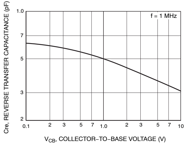
Figure 4. C_{re} - V_{CB}
