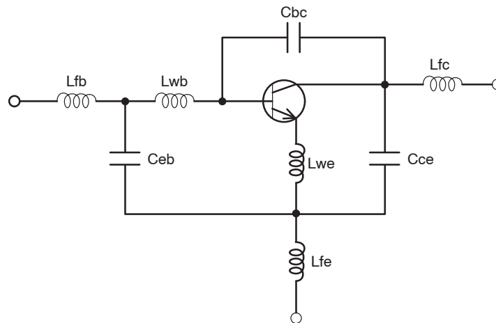
Figure 10. Schematic
