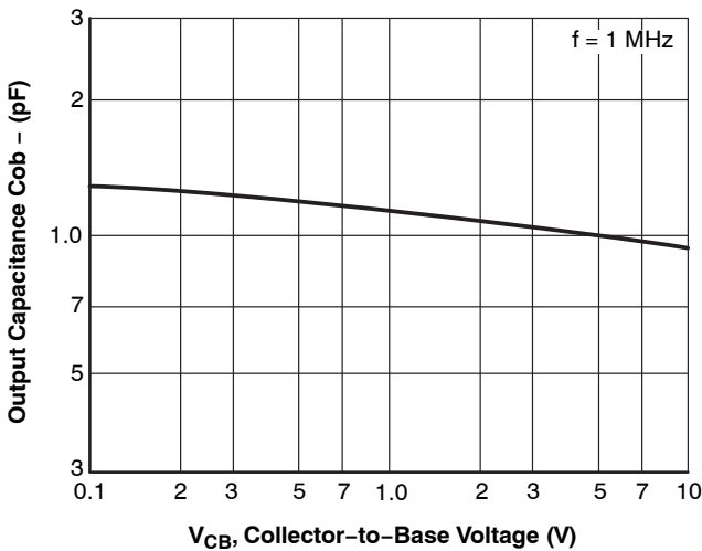
Figure 5. C_{ob} - V_{CB}
