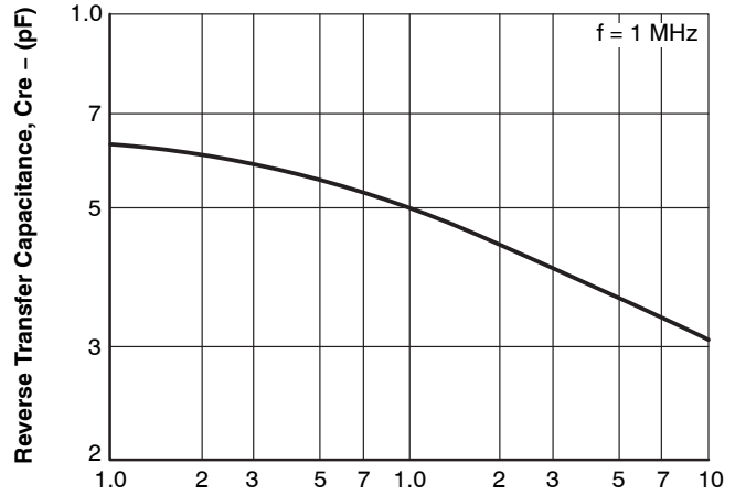
Figure 4. C_{re} - V_{CB}
