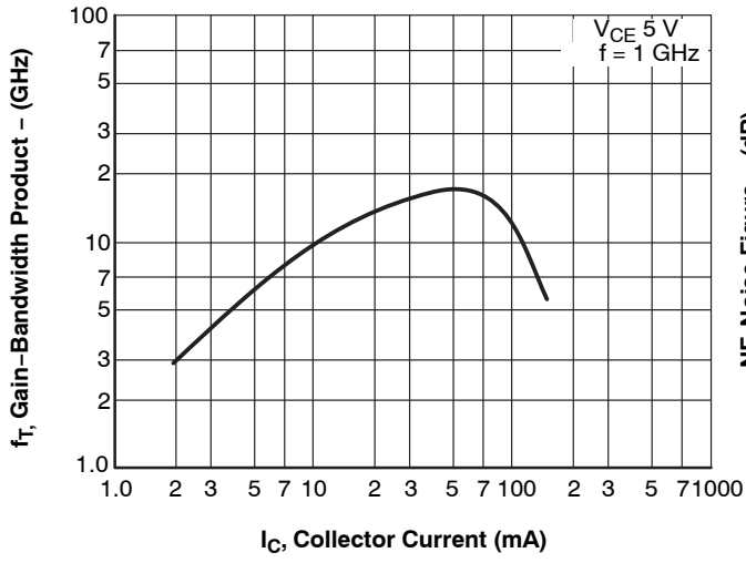
Figure 7. f_T - I_C
