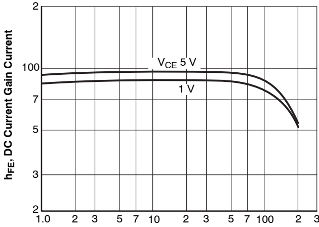
Figure 3. h_{FE} - I_C
