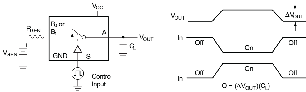
Figure 14. Charge Injection
